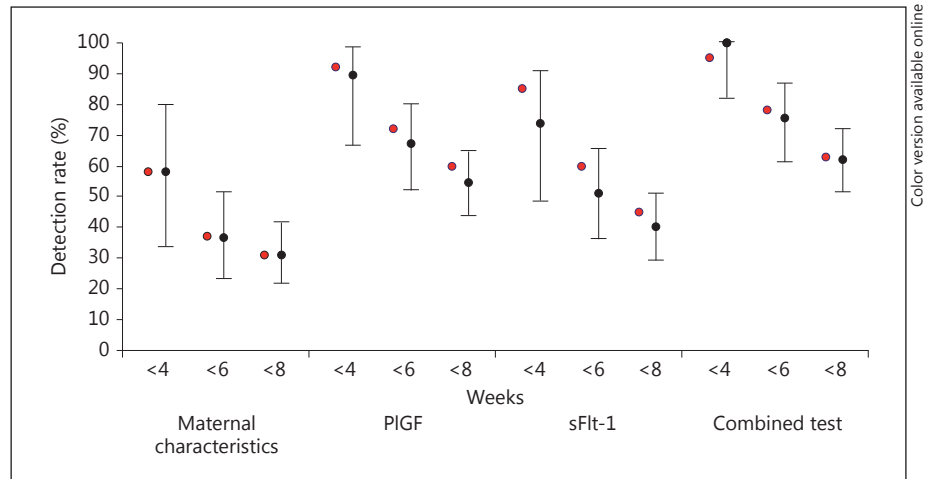
Fig. 2. Empirical DR with 95% confidence interval of PE requiring delivery within 4, 6 and 8 weeks of screening using maternal characteristics alone and maternal characteristics with biochemical markers, at FPR of 5%. The red circles represent the modelled DRs for the same maternal characteristics.
