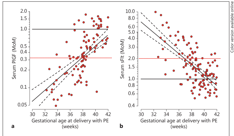
Fig. 1. Scatter diagram and regression line with 95% confidence limits (interrupted lines) for the relationship between PlGF (a) and sFlt-1 (b) MoM at 30–33 weeks' gestational age and interval from screening to delivery in pregnancies with PE. The red horizontal line represents the 5th percentile for PlGF and the 95th percentile for sFlt.
