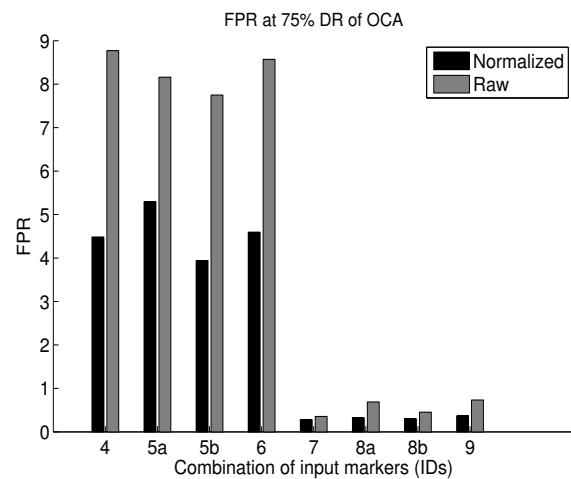
Fig. 6: FPRs of the ANNs built with normalized (black bars) and raw (grey bars) values of Dataset B at a OCA DR of 75%. The results of the different input markers combinations are shown in the x-axis.
