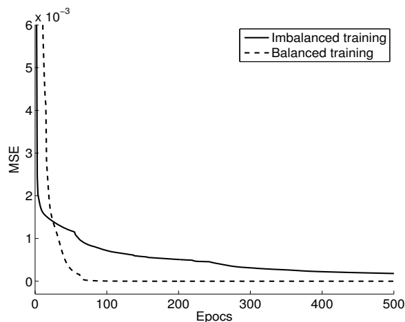
Fig. 3: Mean Squared Error (MSE) of the neural network that was trained for 500 epochs. Dashed and solid lines show the MSE of balanced and imbalanced training sets.
