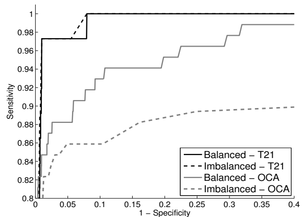
Fig. 7: ROC curves of the models build with balanced (solid lines) and imbalanced (dashed lines) datasets for the euploid-T21 (black lines) and euploid-OCA (grey lines). The data are referred to the 7 markers group and raw data.
